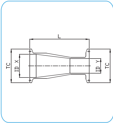
31-14MP - CONCENTRIC REDUCER TC x TC ASME BPE DT-4.1.3-3
