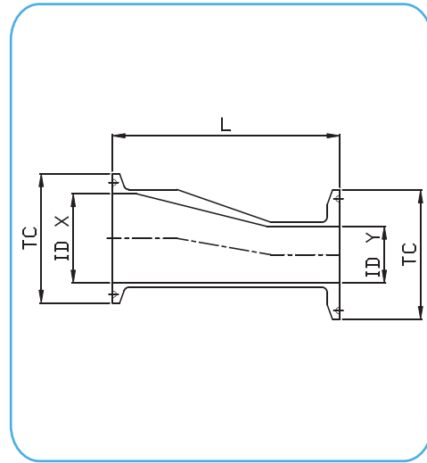
32-14MP - ECCENTRIC REDUCER TC x TC ASME BPE DT-4.1.3-3
